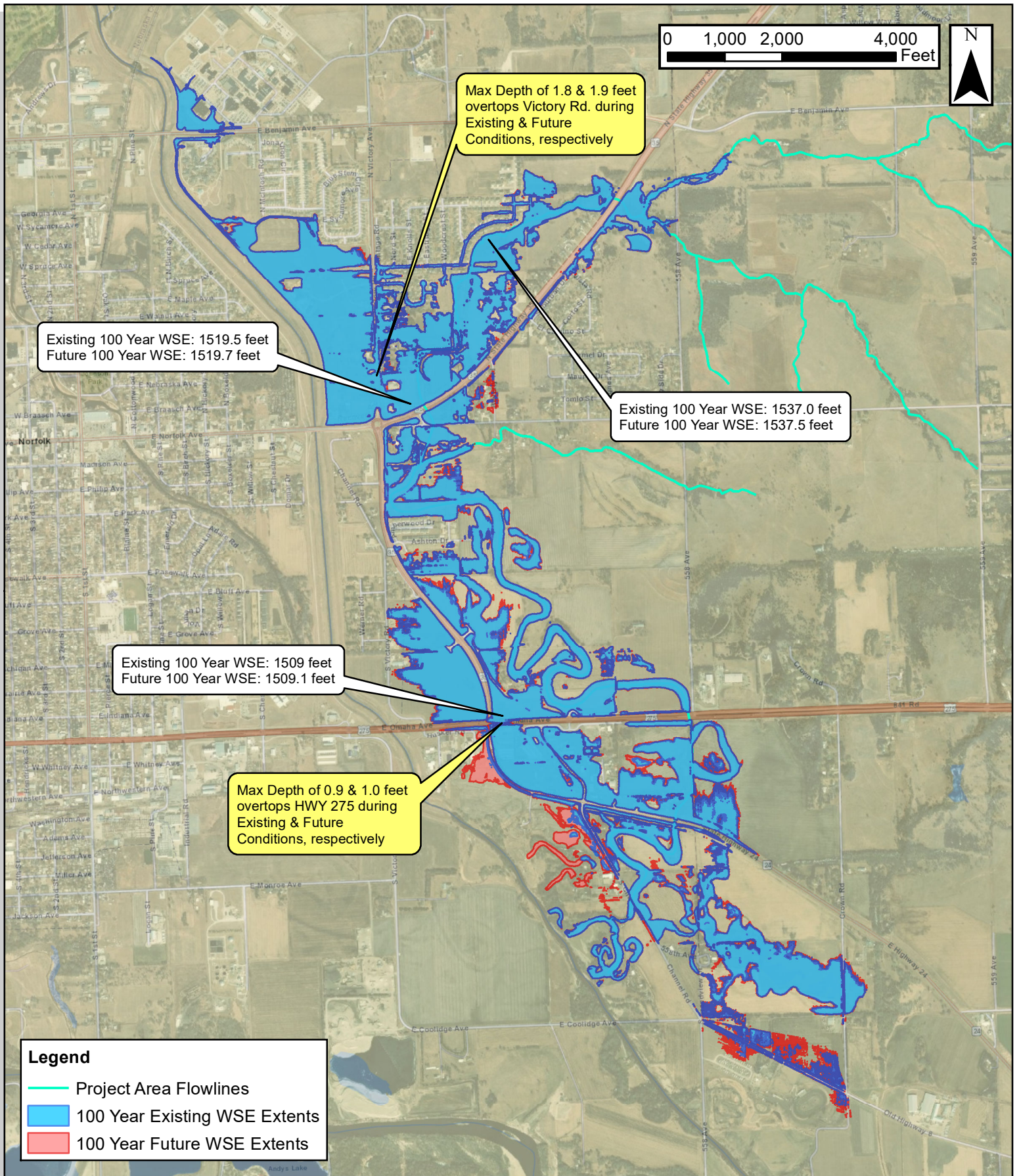
Figure 11: 100-Year Existing vs. Future WSE Extents - Closed Outlets
