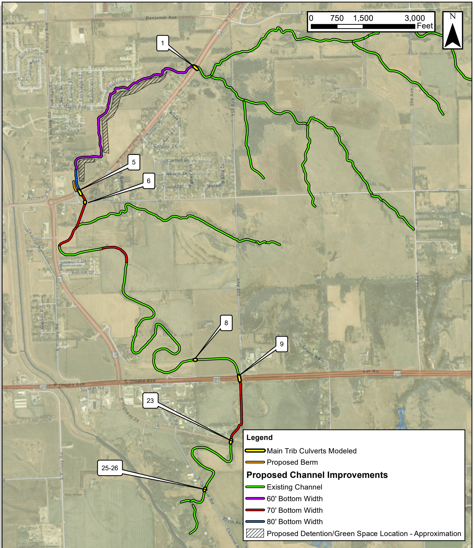
Figure 12: Proposed Structural Improvement Location and Sizing
