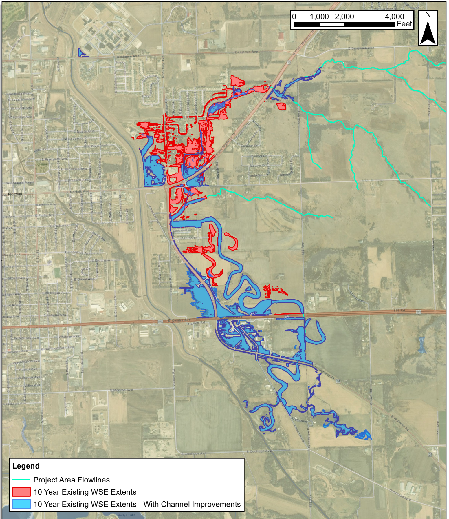
Figure 13: Existing Conditions with Channel Improvement - Open Outlets
