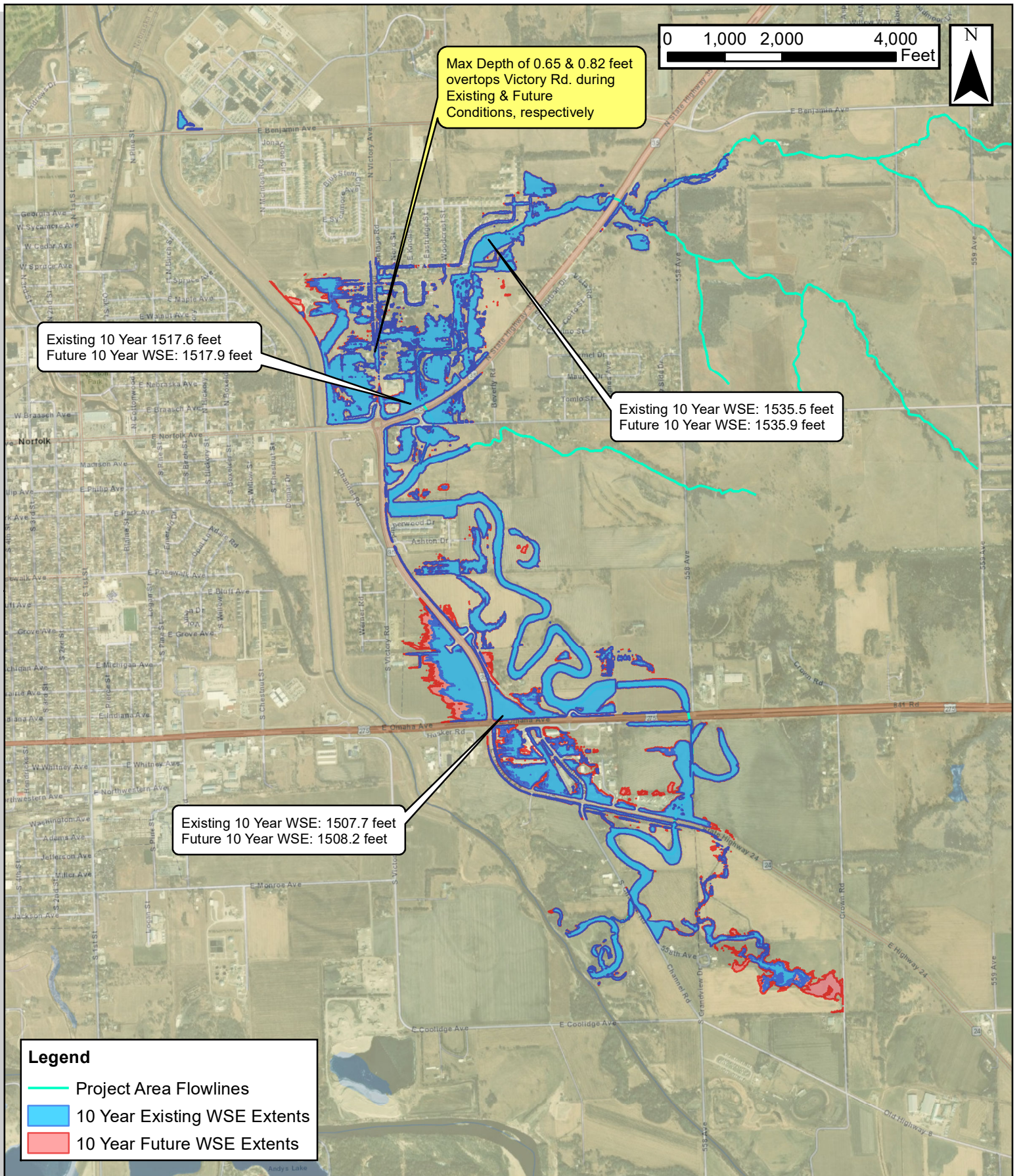
Figure 7: 10-Year Existing vs. Future WSE Extents - Open Outlets
