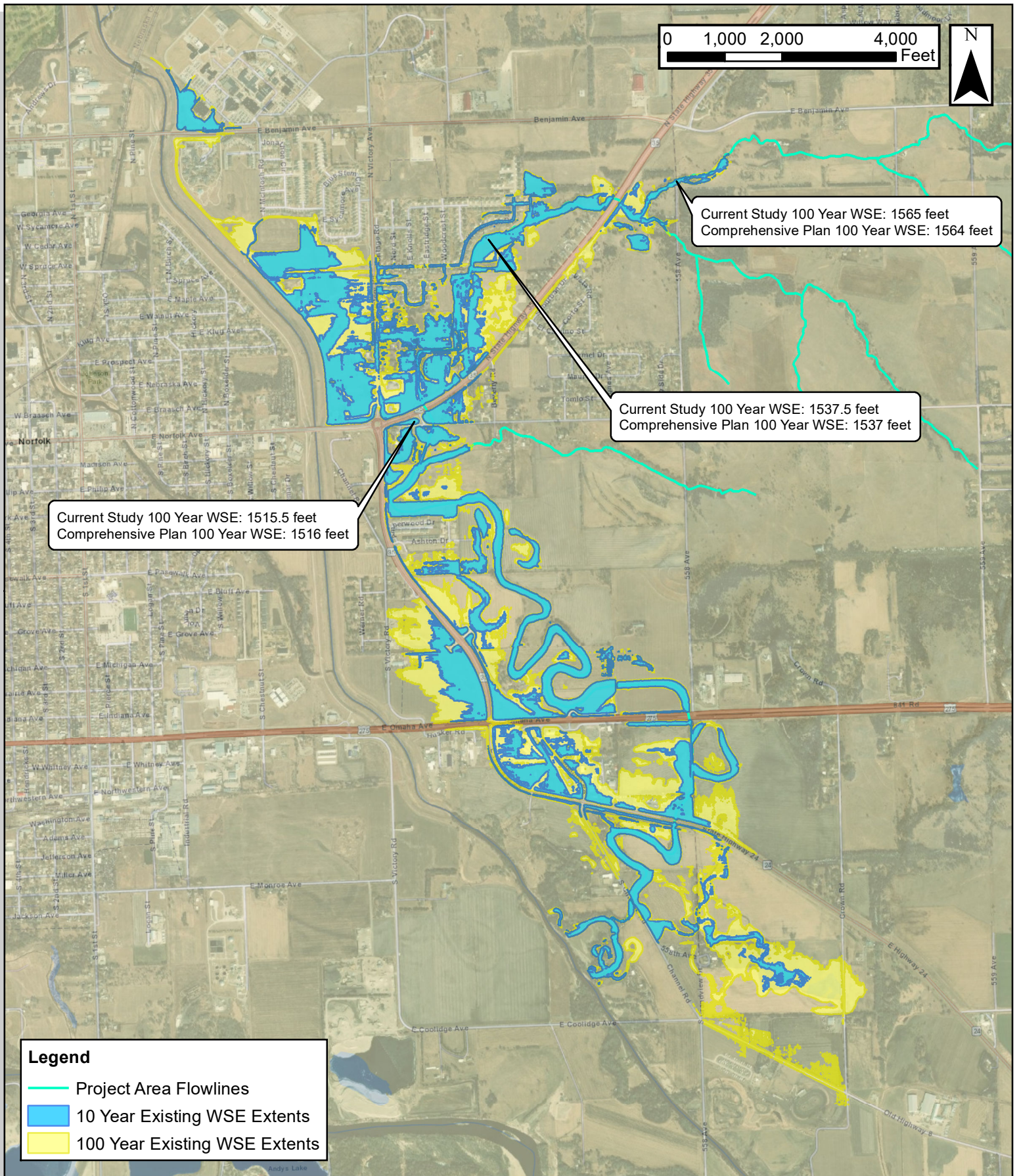
Figure 9: Existing Conditions WSE Extents - Closed Outlets
