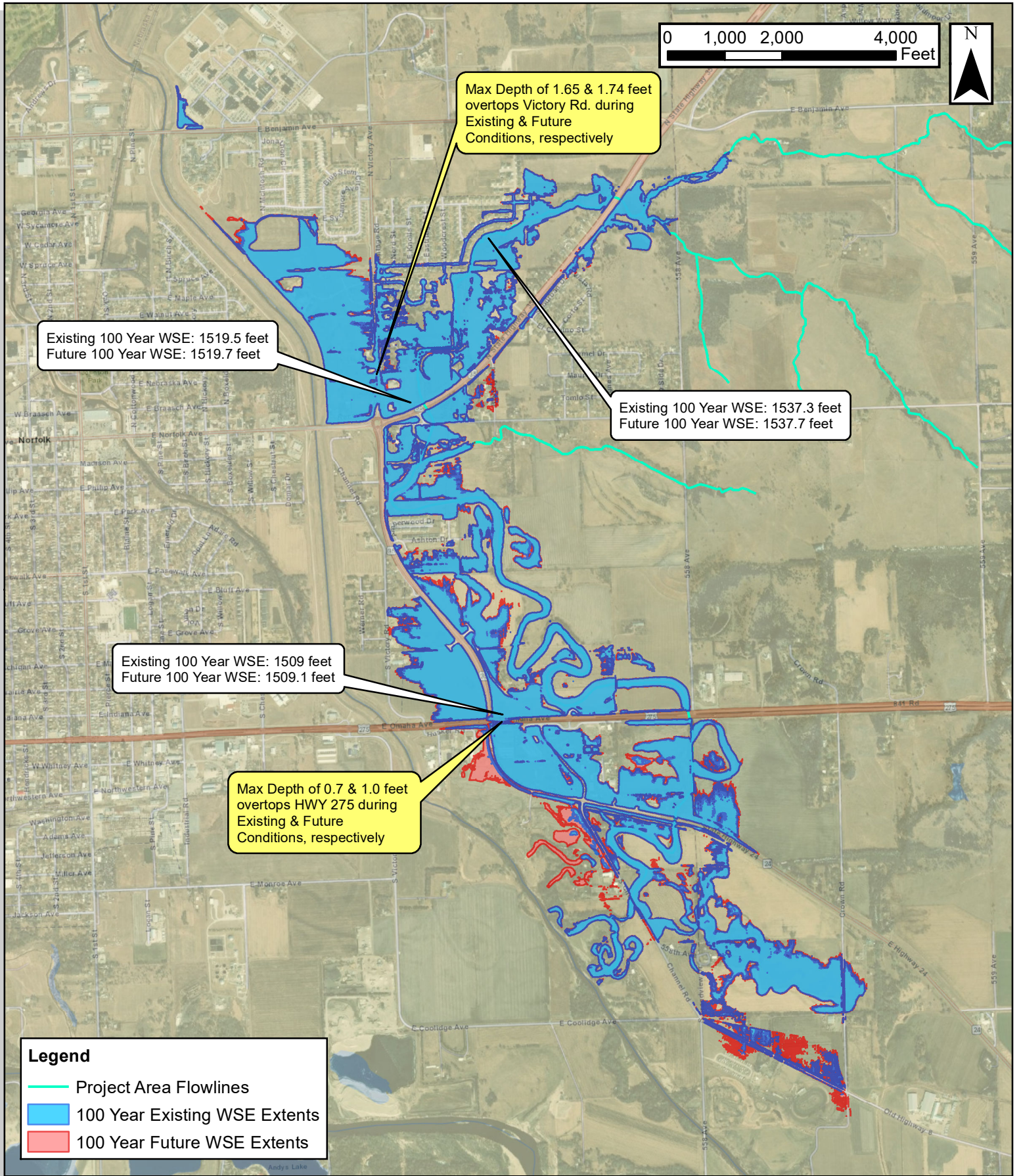
Figure 8: 100-Year Existing vs. Future WSE Extents - Open Outlets
